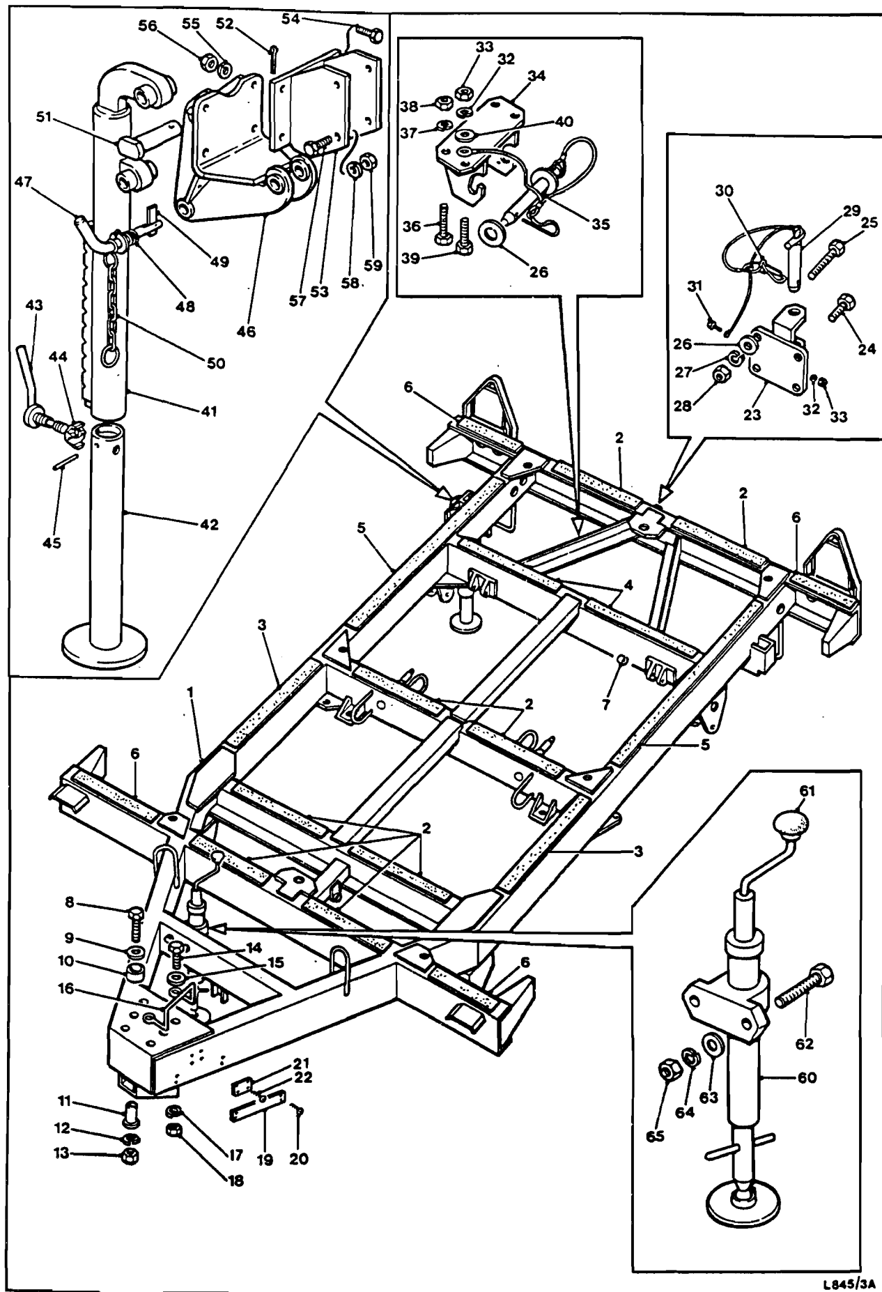
Fig.1 Chassis
