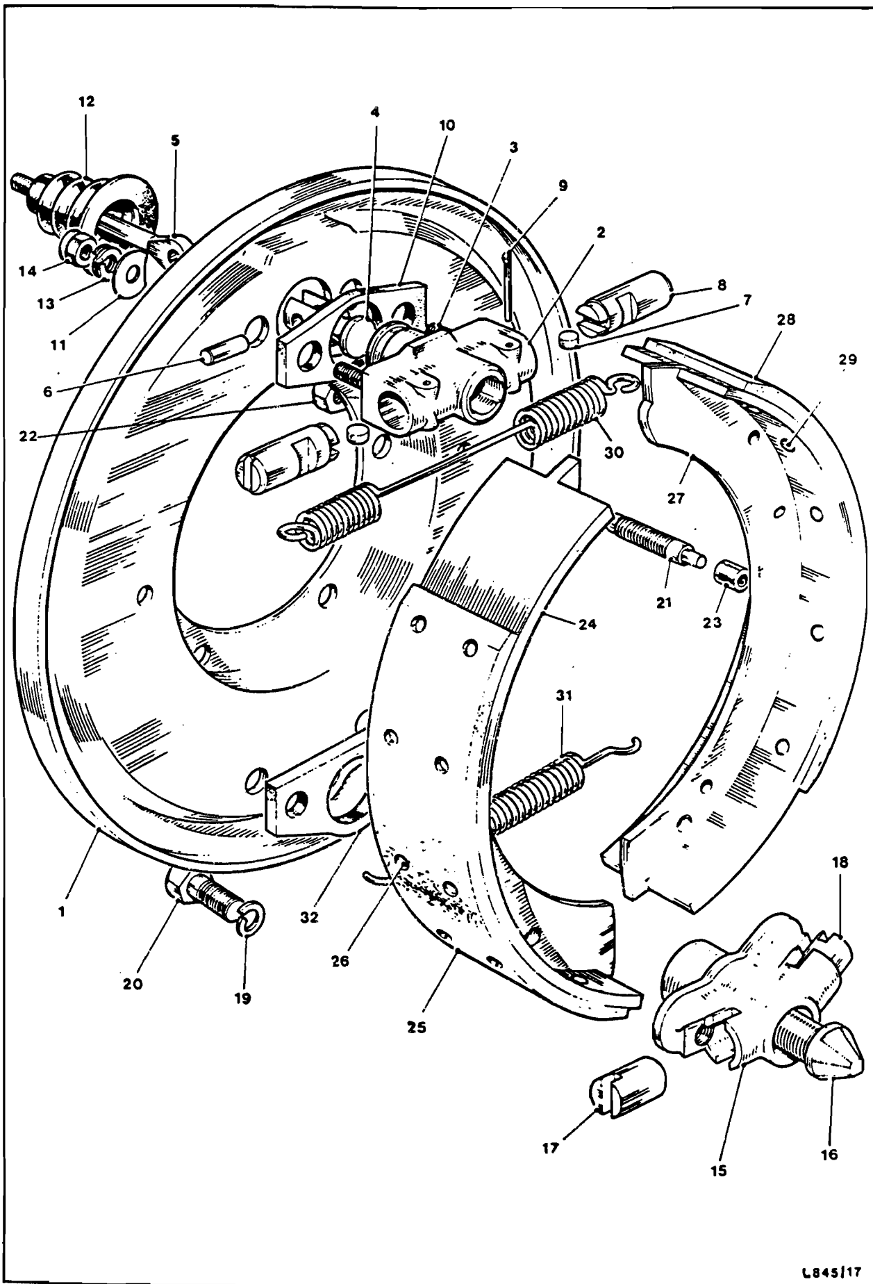
Fig.5 Brake
