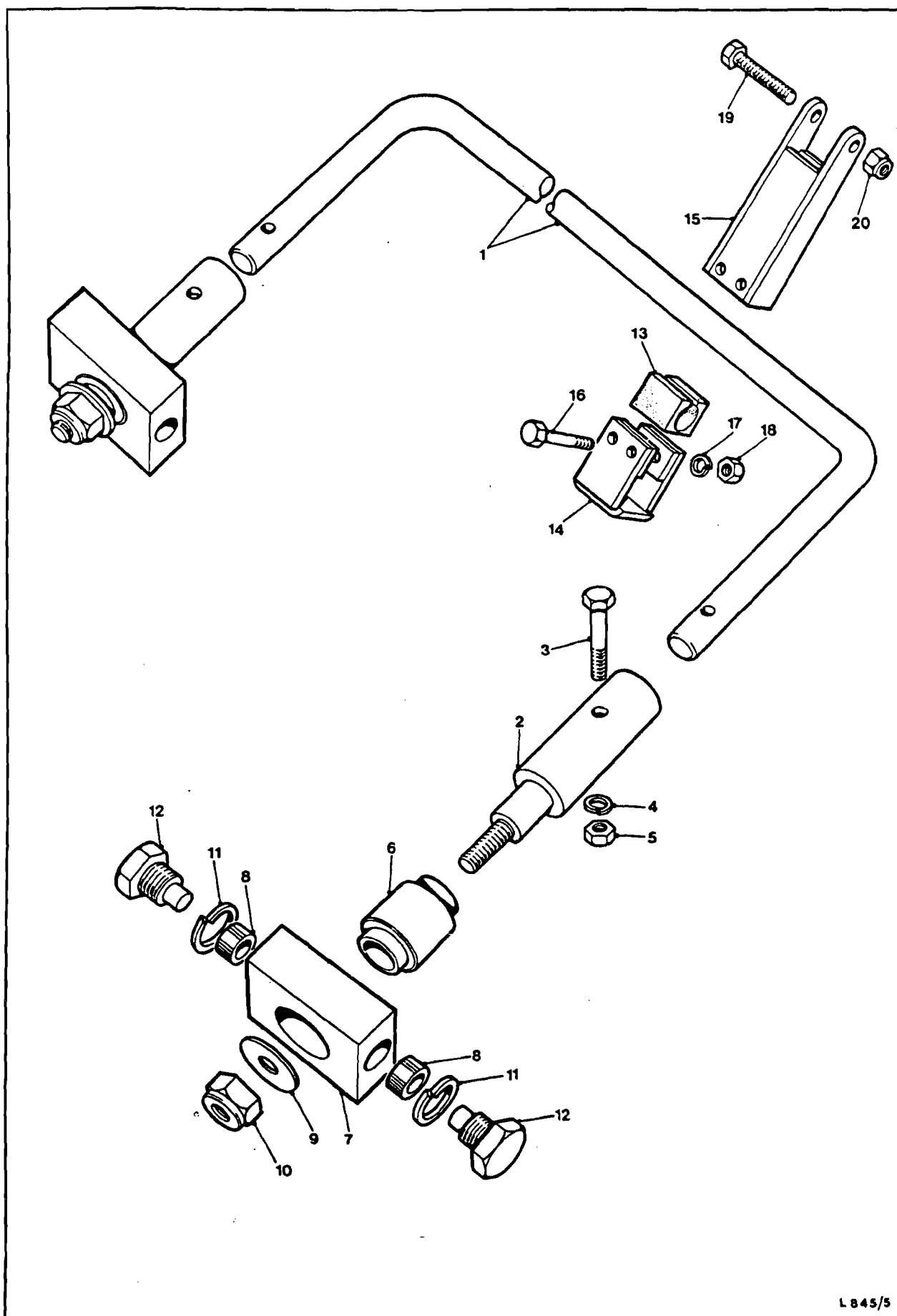
Fig.3 Anti-roll bar
