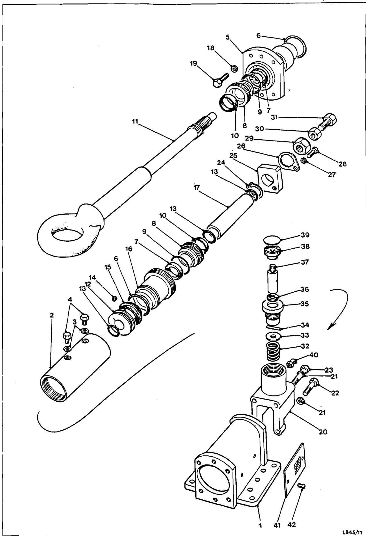
Fig.9 Hydraulic damper and draft eye
