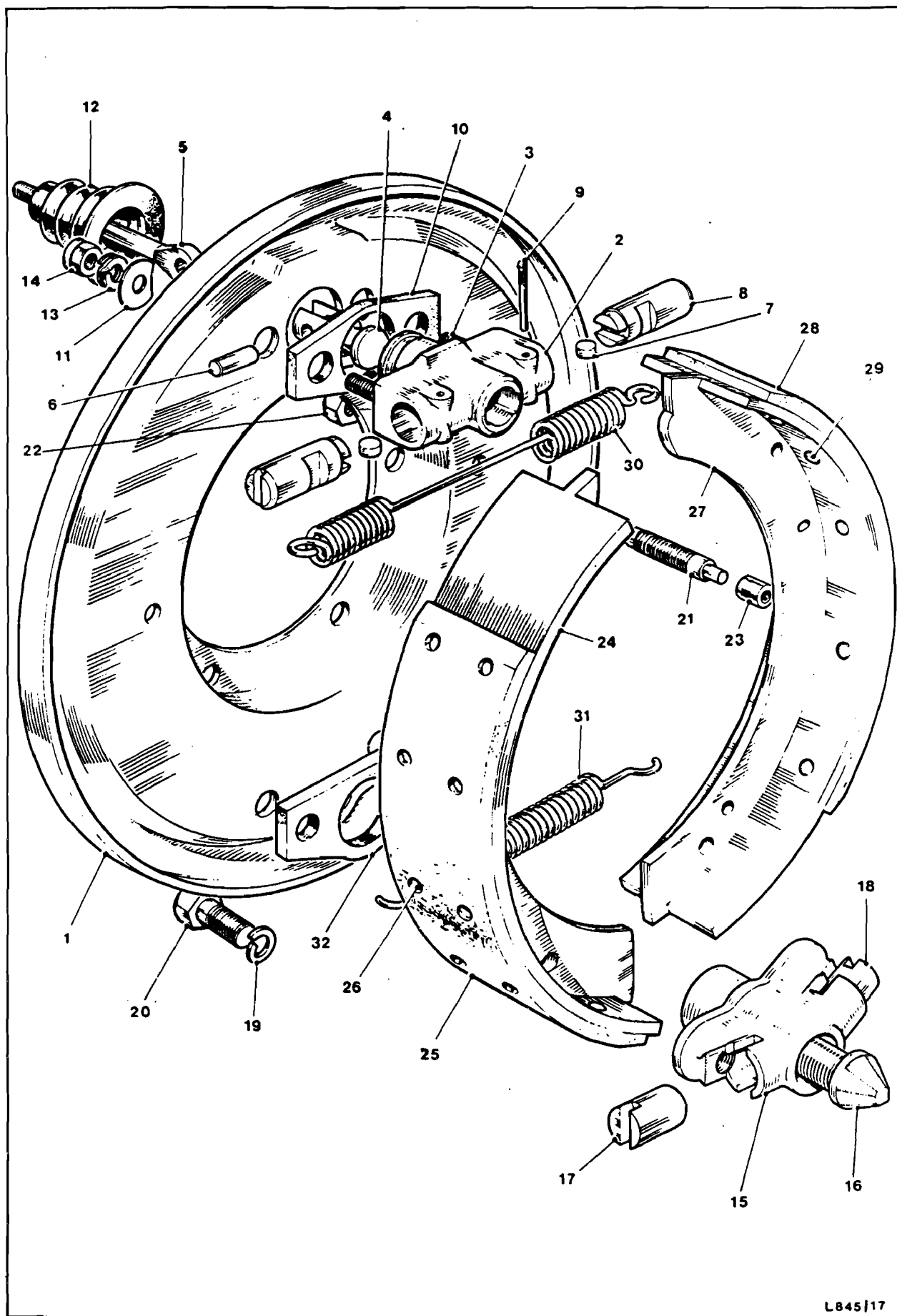
Fig.5 Brake
