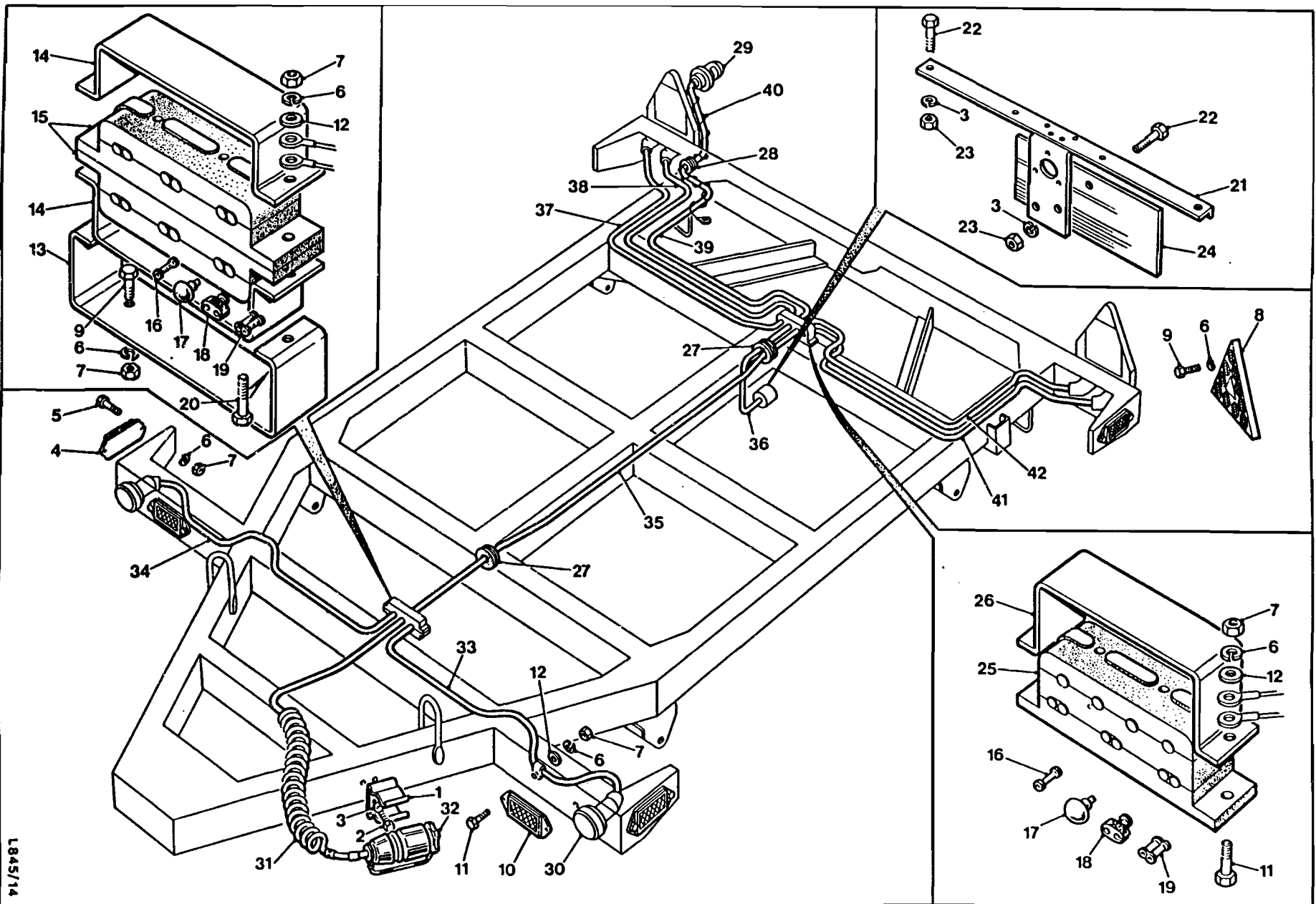
Fig.12 Electrical wiring
