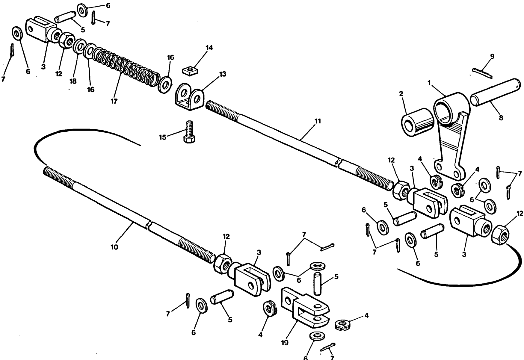
Fig.7 Brake linkage
