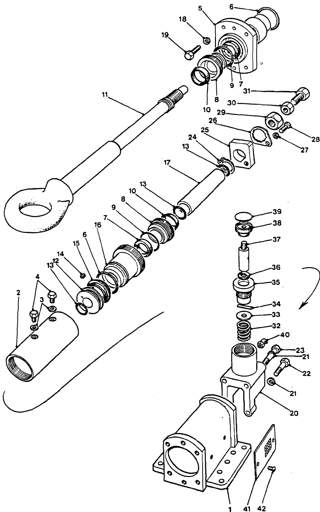
Fig.9 Hydraulic damper and draft eye
