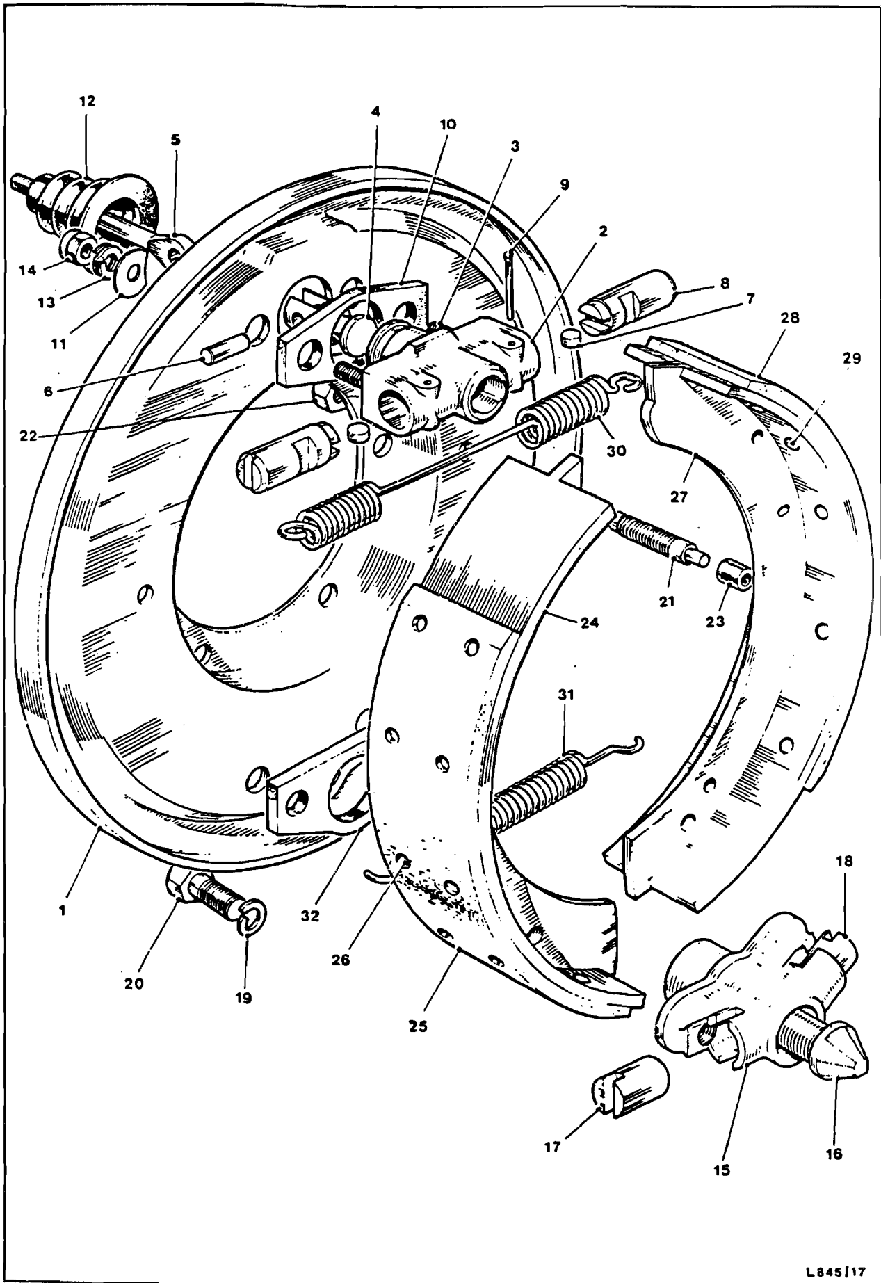
Fig.5 Brake
