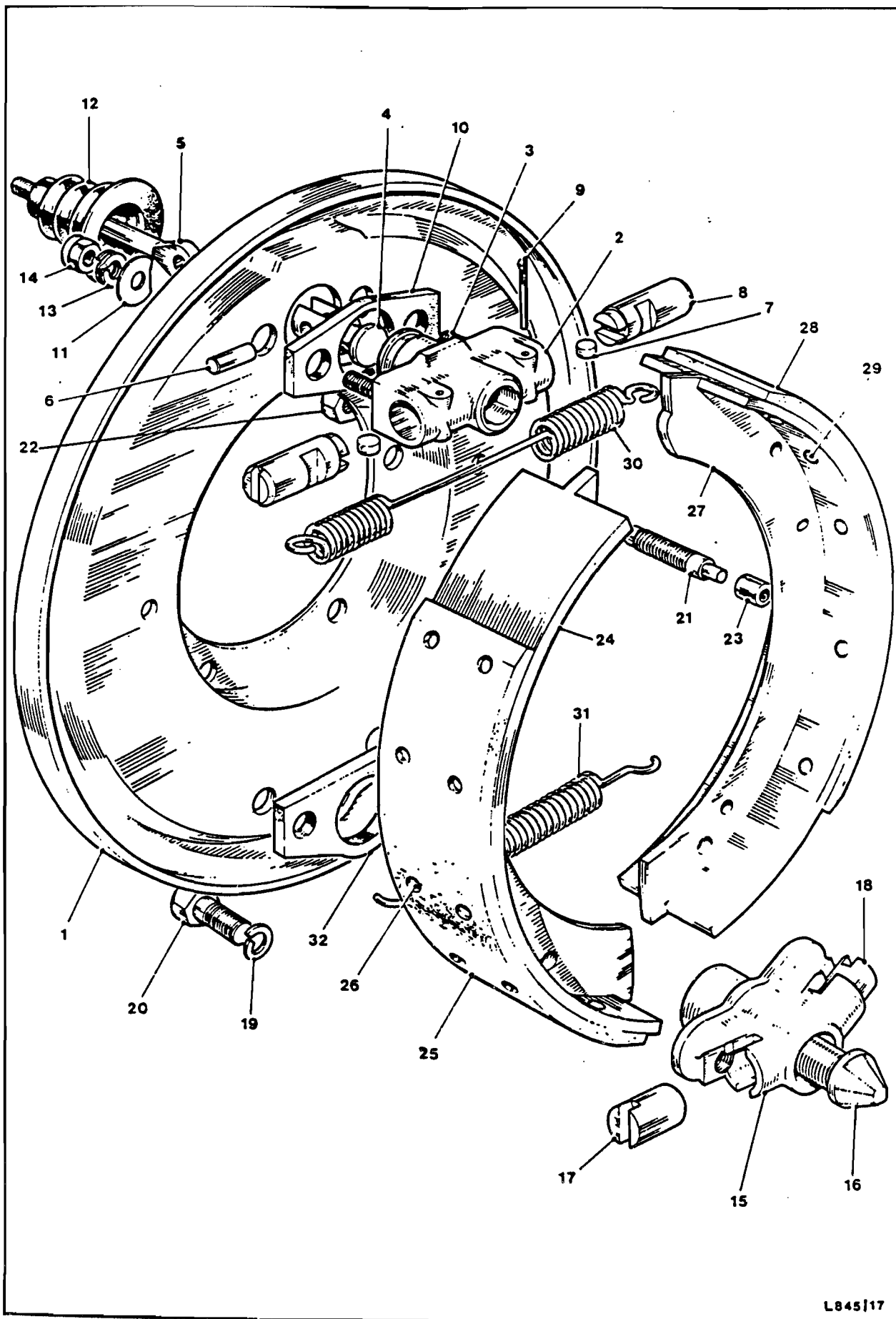
Fig.5 Brake
