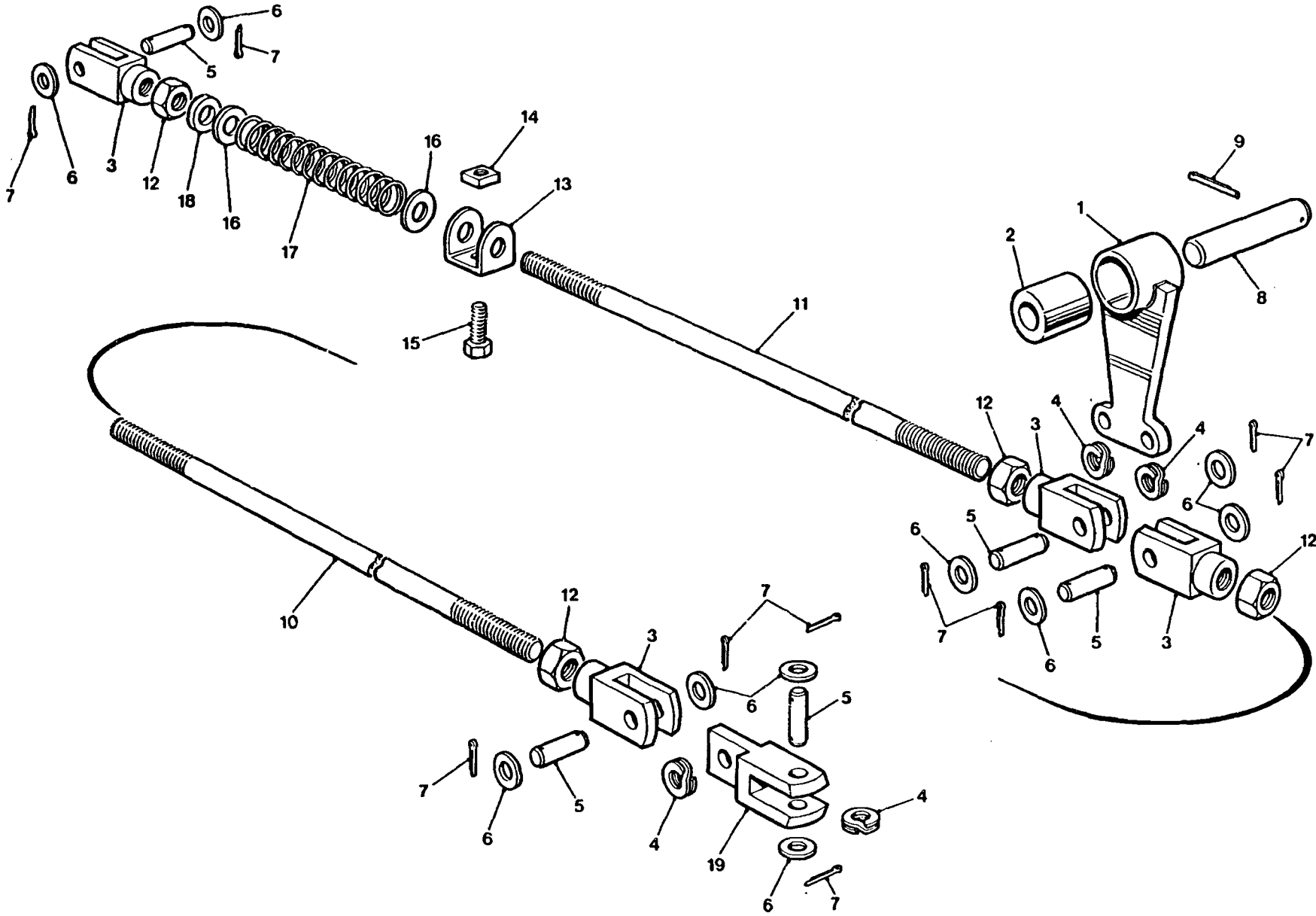
Fig.7 Brake linkage
