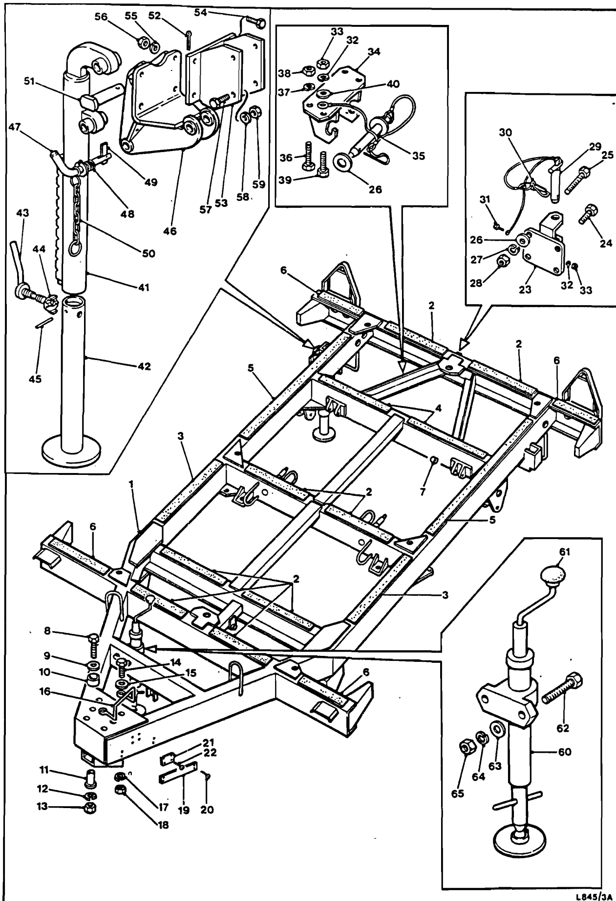
Fig.1 Chassis
