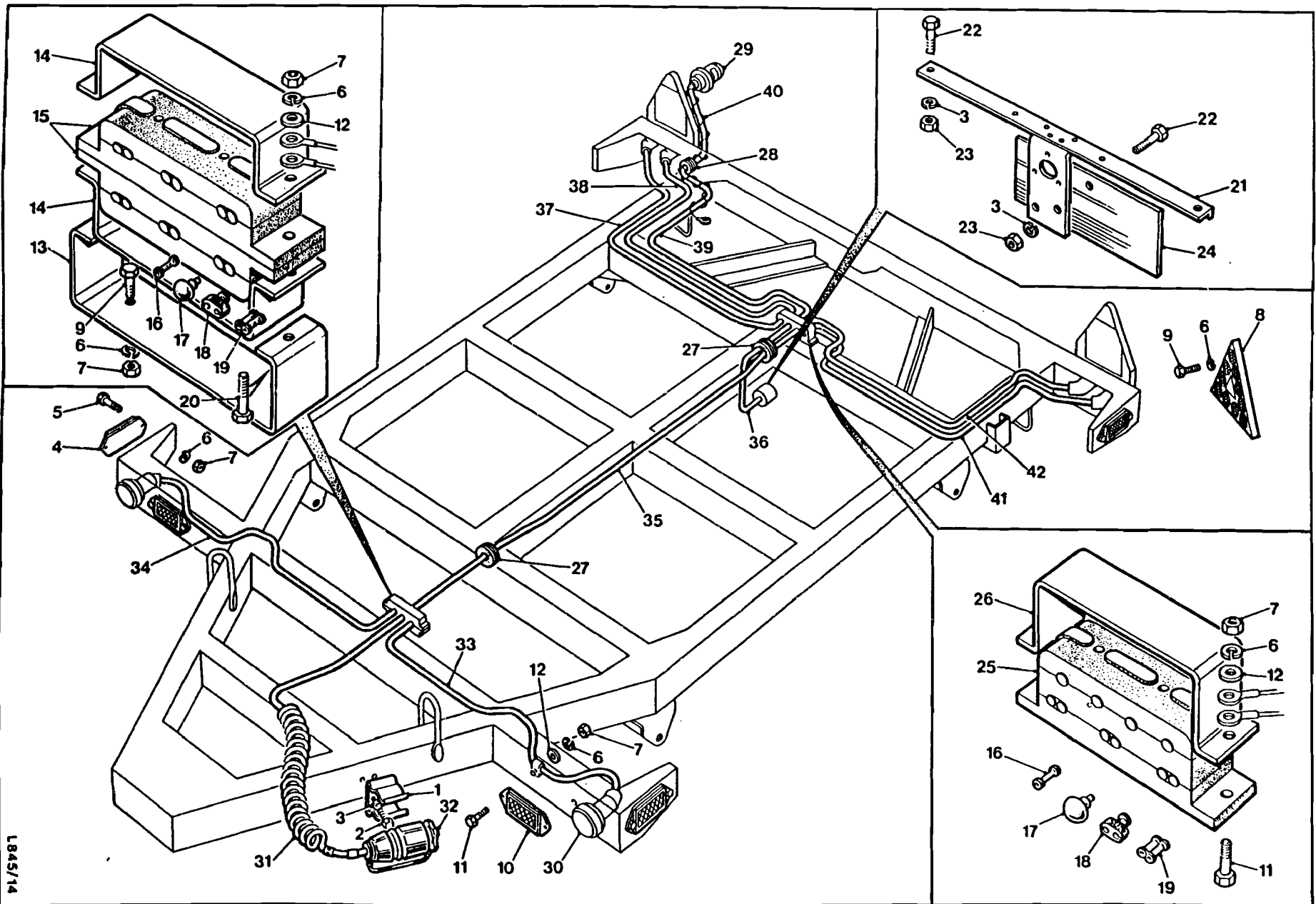
Fig.12 Electrical wiring
