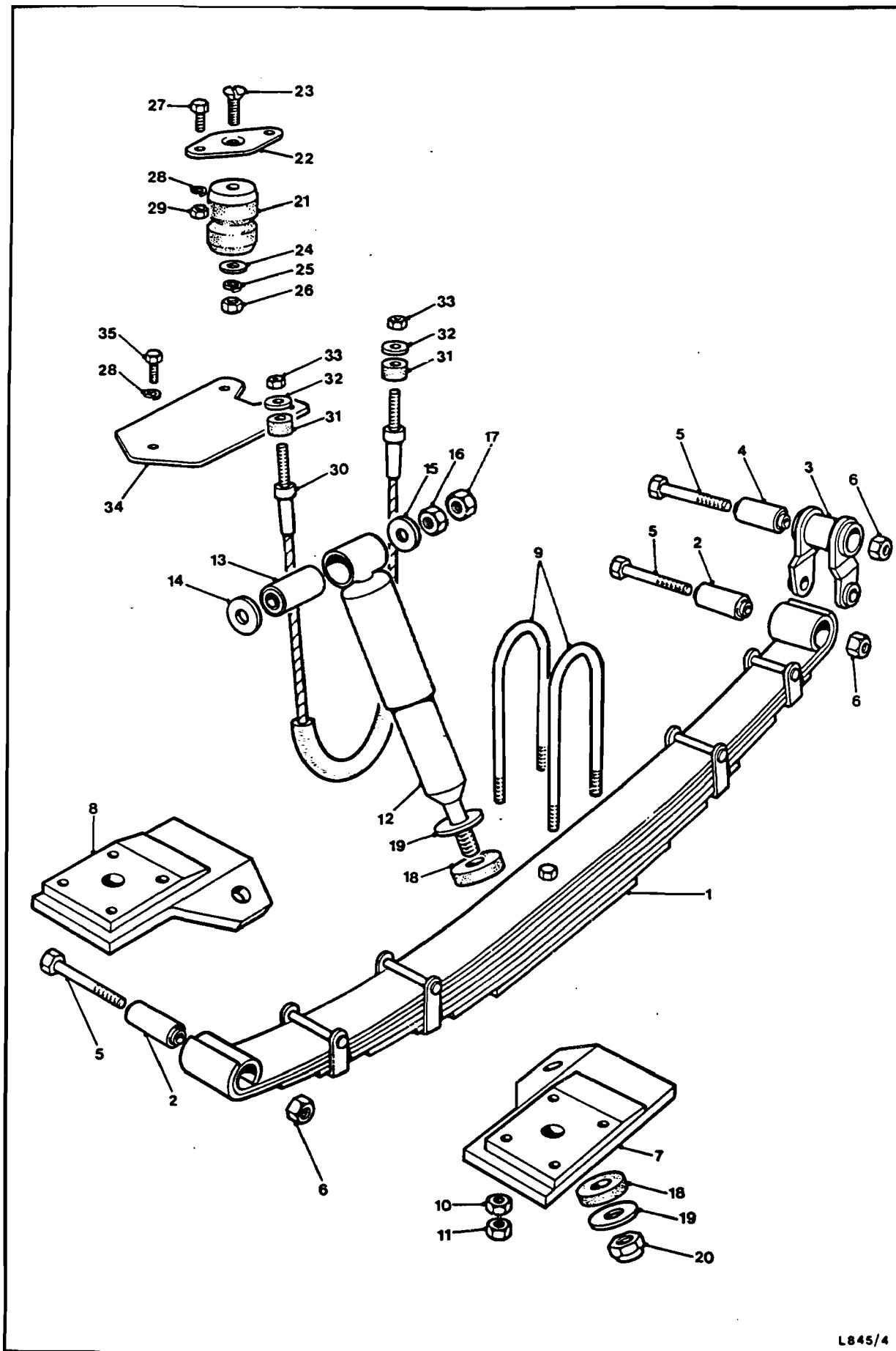
Fig.2 Suspension
