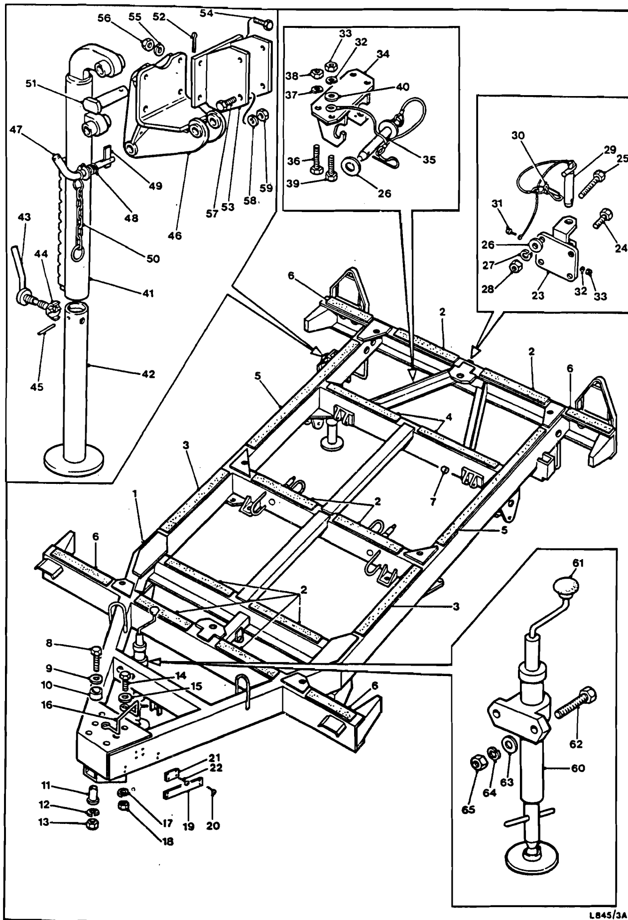
Fig.1 Chassis
