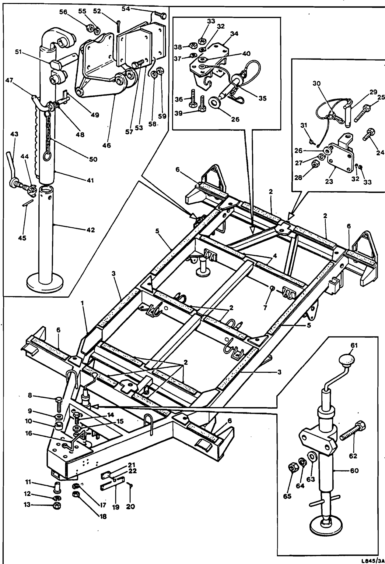
Fig.1 Chassis
