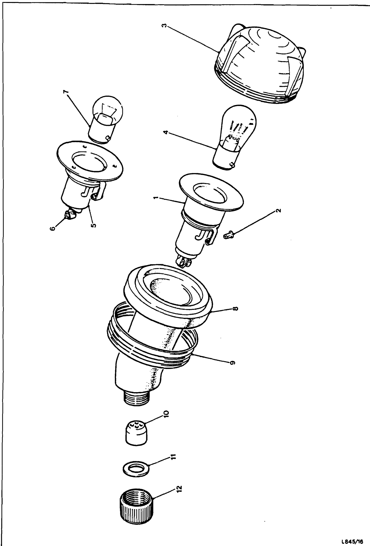
Fig.14 Side, turn and taillight
