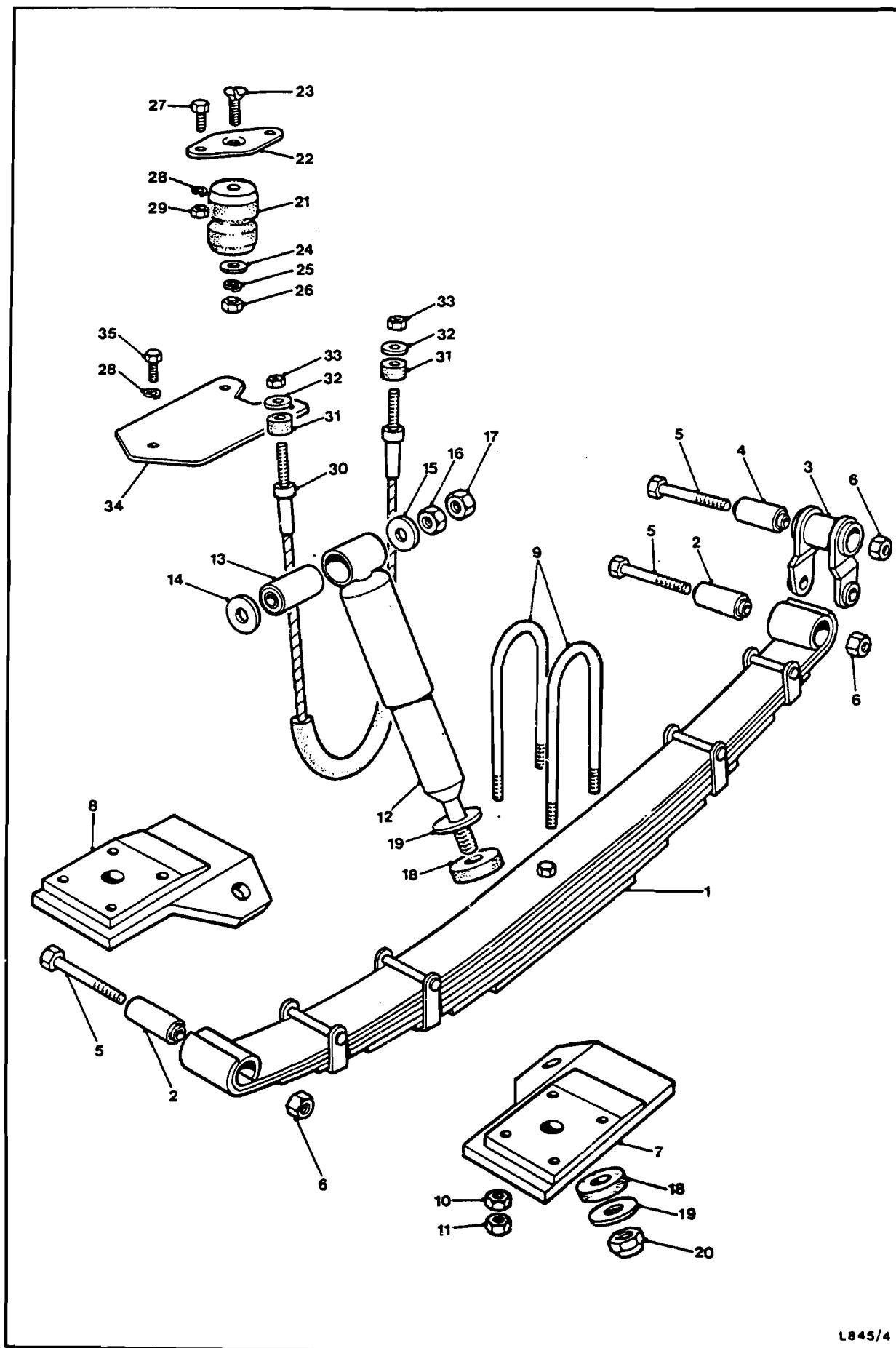
Fig.2 Suspension
